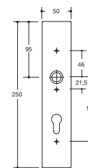
Schild 236.21X..
