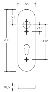
Schild 285...
