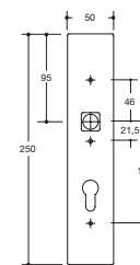
Schild 236.20SX..
