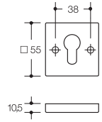
Schlüsselrosette 308X..
