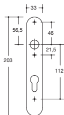
Schild 219.21X..H
