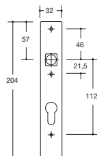
Schild 220.20SX..
