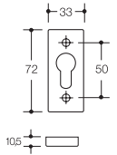
Schlüsselrosette 318X.../FS
