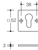
Schlüsselrosette 308XAL
