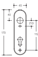
Schild 230...X..
