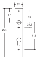
Schild 220.21X..
