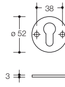
Schlüsselrosette 306.23XAL
