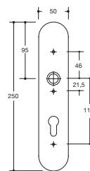
Schild 235.21X..
