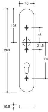
Schild 235...
