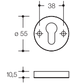
Schlüsselrosette 306.23X..
